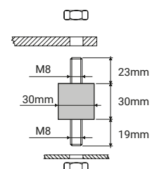
Vibration absorber
