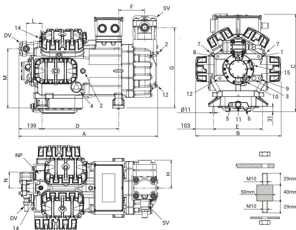
Vibration absorber
