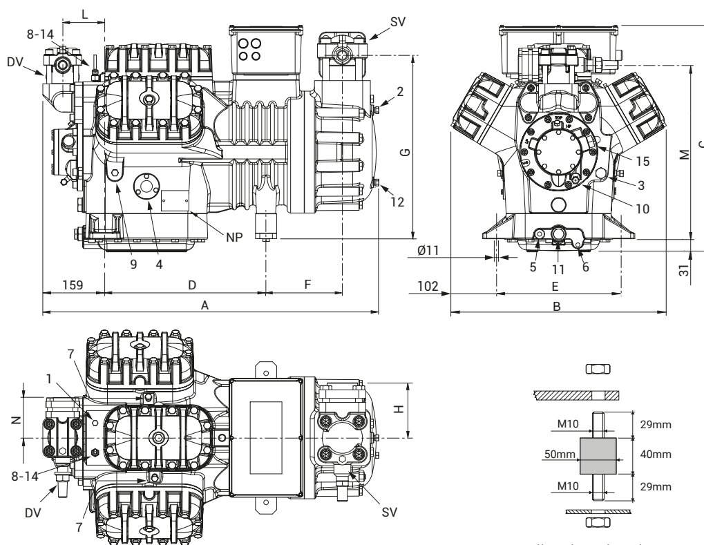
Vibration absorber
